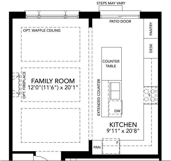
Opt. Main Level With Entertainer's Kitchen ELEV. A
