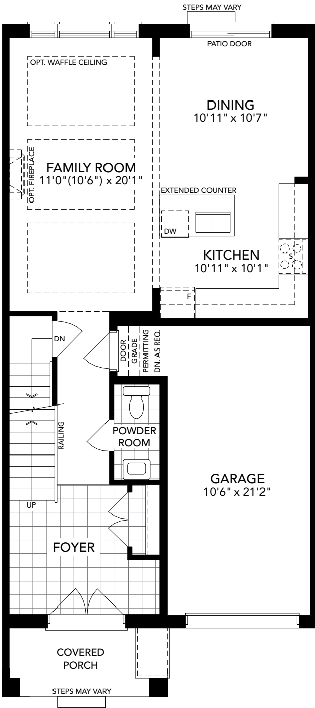
Main Level ELEV. A
