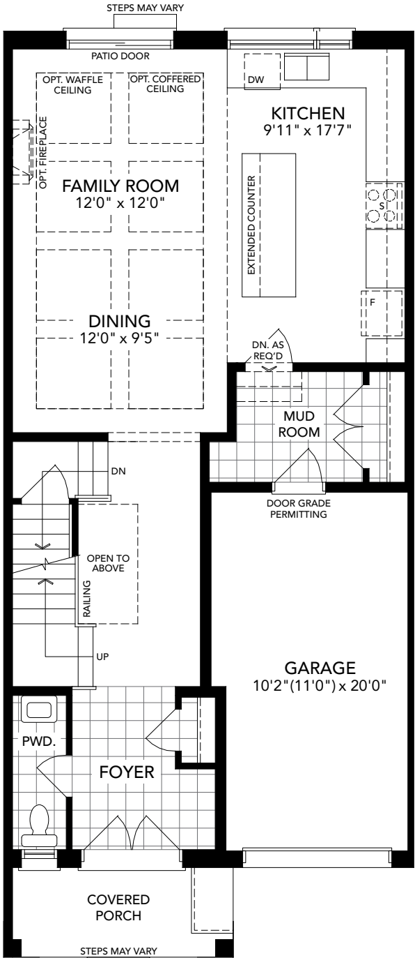
Opt. Main Level ELEV. A
