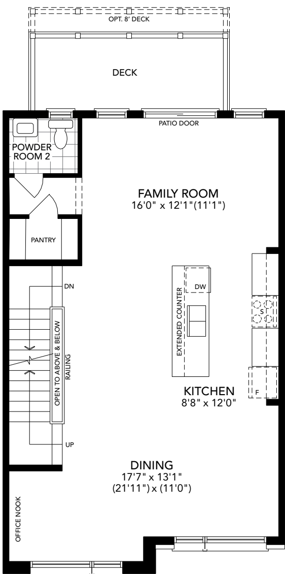
Main Level ELEV. A
