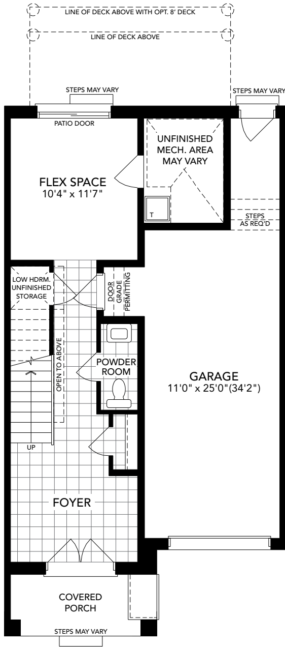
Ground Level ELEV. A
