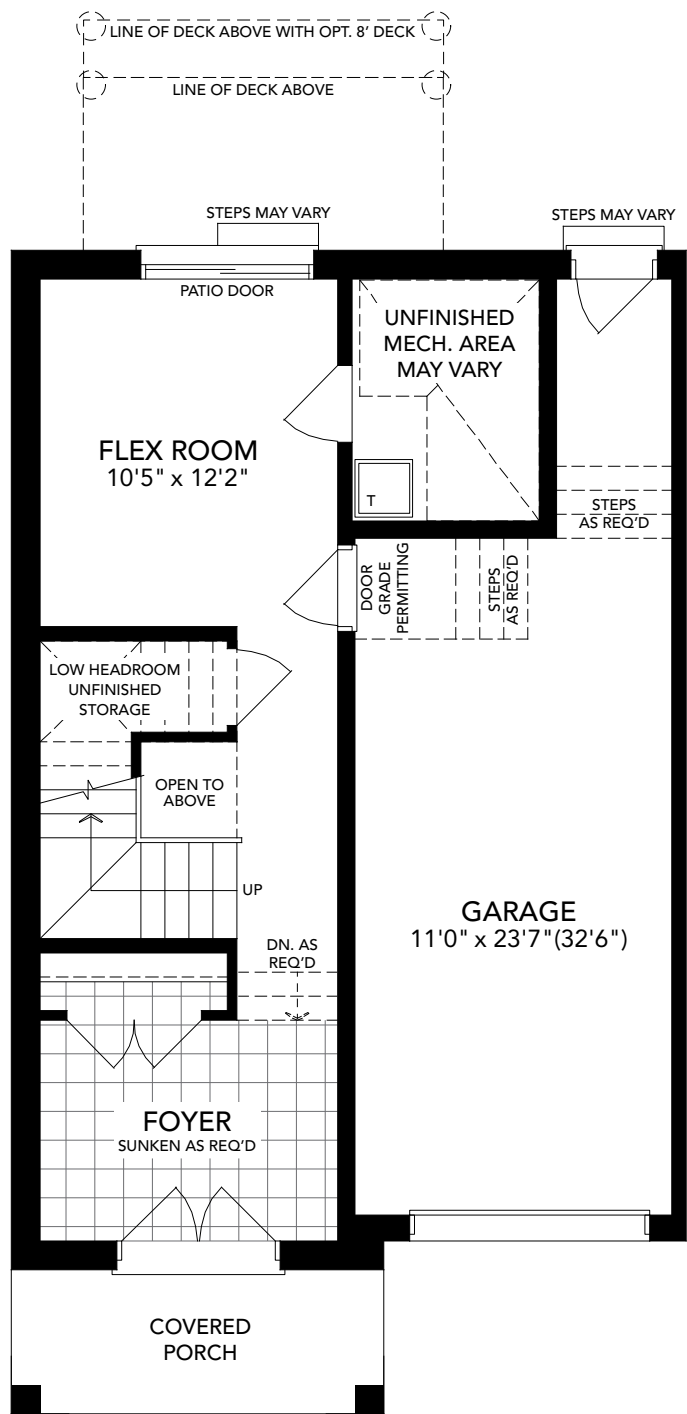
Ground Level ELEV. A
